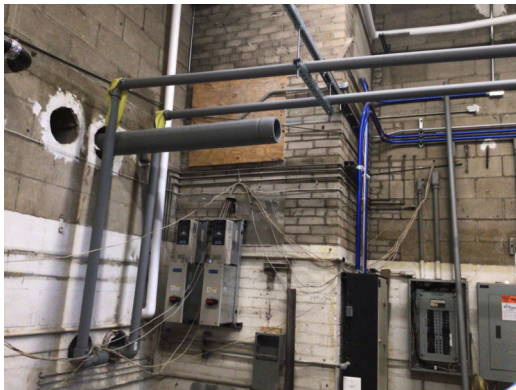
Central Ed. – Hydronic piping installation in the lower-level.
